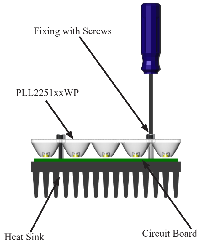
PLL2251xx - With Screws
